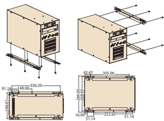
Bidirectional mounting
